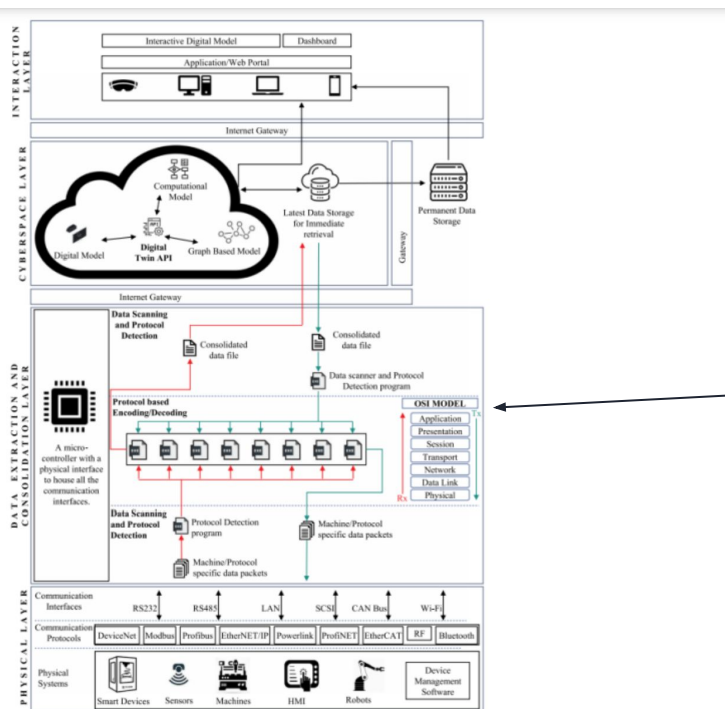
Figure 3.8: four-Layered CPS architecture for building the DT (Zheng & Sivabalan, 2020).
